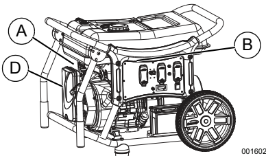
Figure 3-2. Engine Controls
