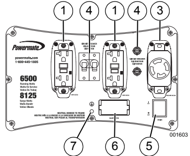
Figure 2-2. CX6500E Control Panel
